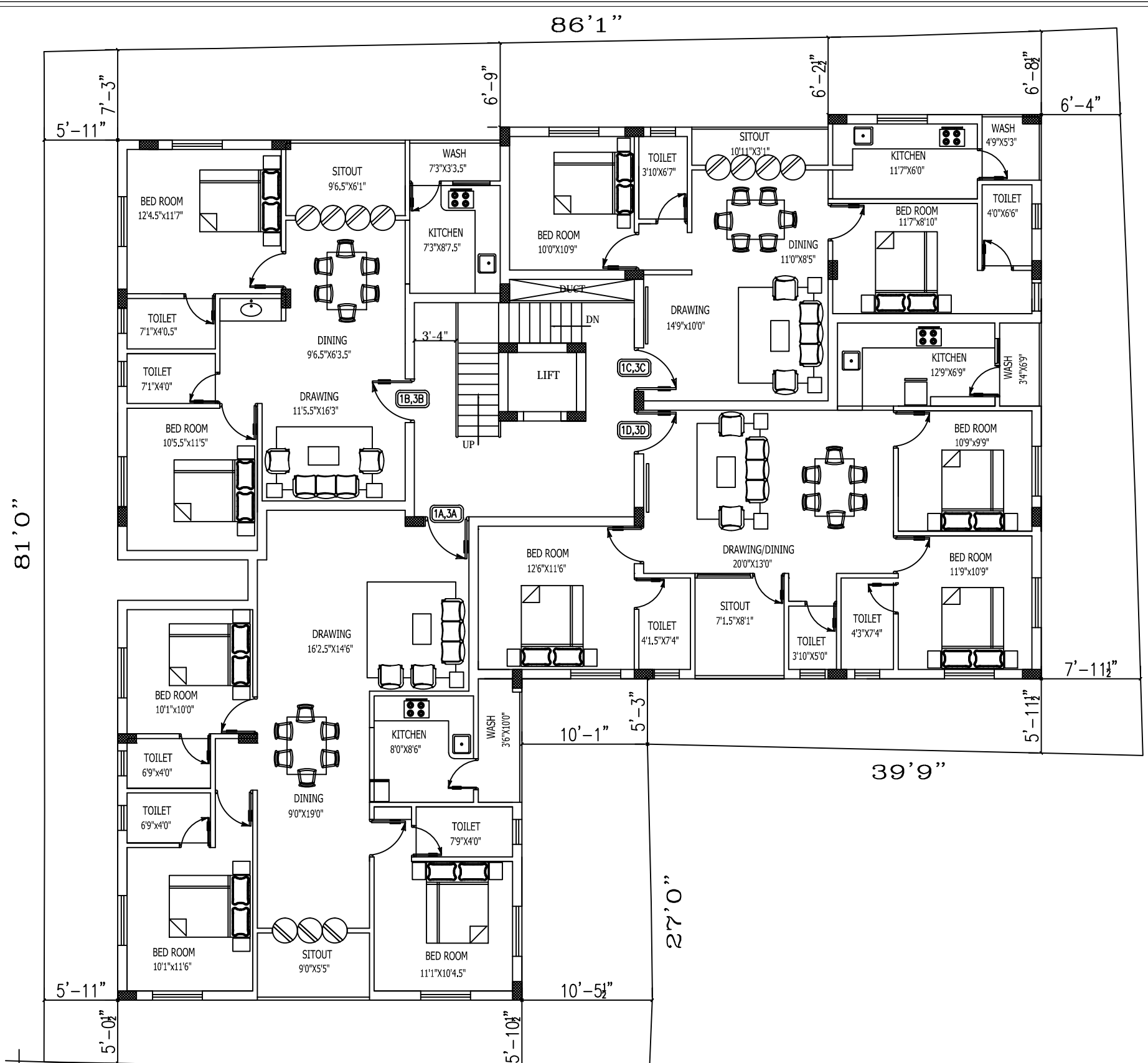
TYPICAL 1ST & 3RD FLOOR PLAN
